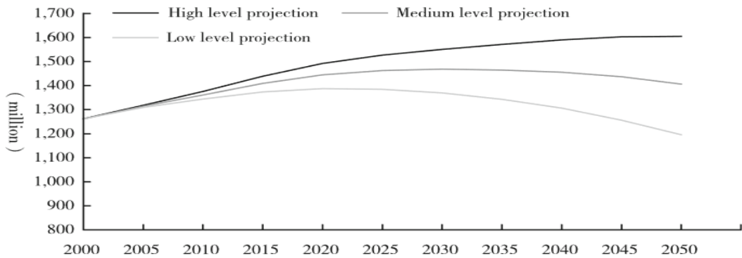
Fig. 6 Three demographic projections during 2000–2050
