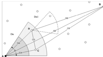
Figure.5. Illustration of the FBR protocol: nodes within the transmitter's cone \theta are candidate relays [Jornet, Stojanovic, and Zorzi, 2008].
