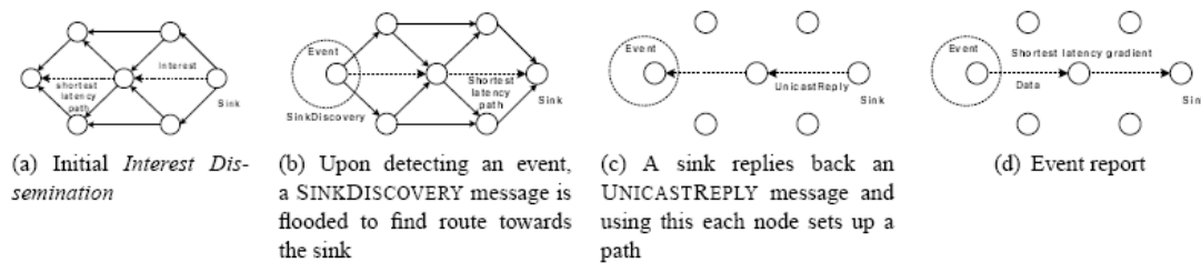
Figure 8. Under-Water Diffusion: Delayed Report Protocol (DRP) [Lee et al., 2006].
