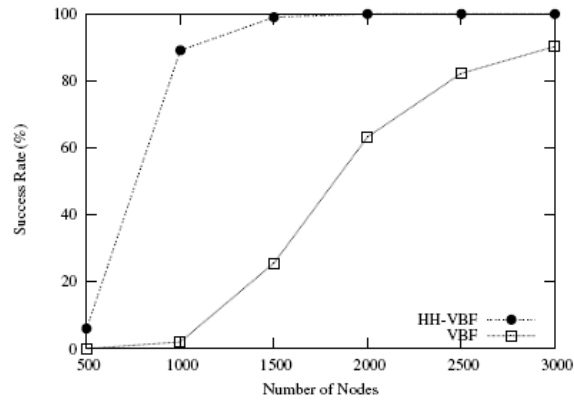
Figure 12a. VBF vs. HH-VBF according to success rate [Xie, Cui, and Lao, 2006]
