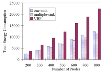
Figure 11(b). DBR vs. VBF according to total energy consumption [Xie, Cui, and Lao, 2006]
