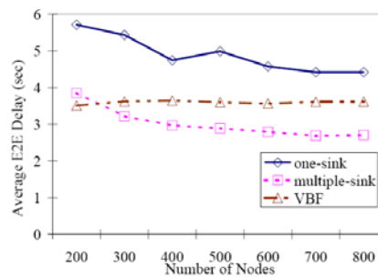
Figure 11(c). DBR vs. VBF according to average end to end delay [Xie, Cui, and Lao, 2006]
