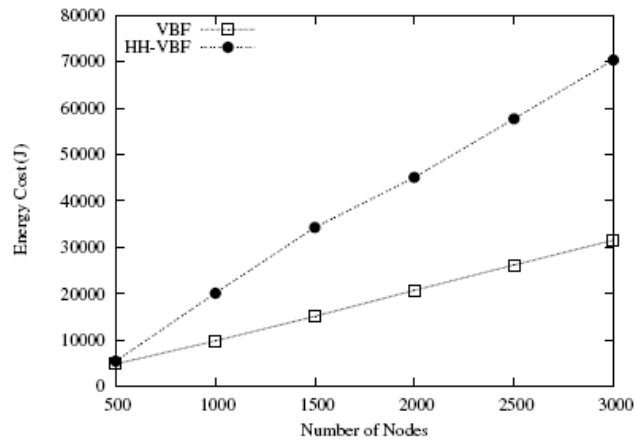
Figure 12b. VBF vs. HH-VBF according to energy cost [Xie, Cui, and Lao, 2006]
