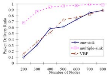
Figure 11(a). DBR vs. VBF according to packet delivery ratio [Xie, Cui, and Lao, 2006]
