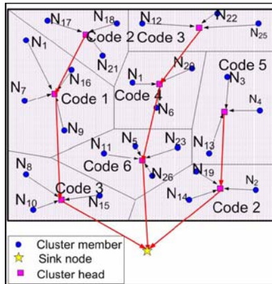
Figure 6. A network case using DUCS [Domingo and Prior, 2007]
