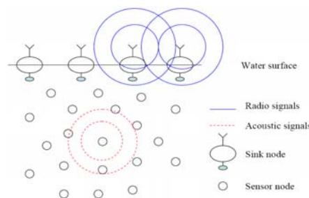
Figure 2. Multiple-sink underwater sensor network architecture [Yan, Shi, and Cui, 2008]
